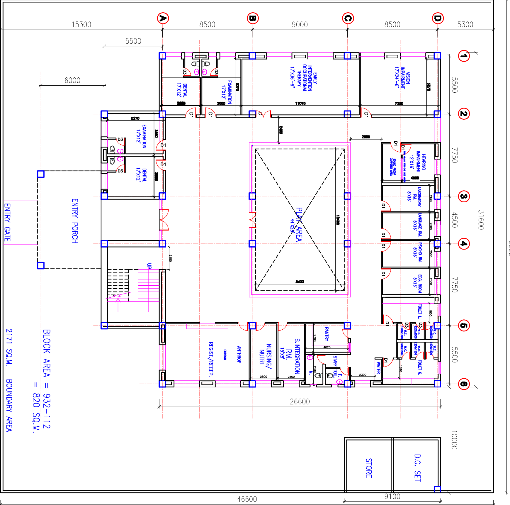
OPTION PLAN-2
